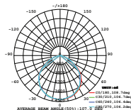
LUMINOUS INTENSITY DISTRIBUTION DIAGRAM
