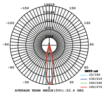
LMINOUS INTENSITY DISTRIBUTION
