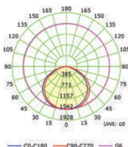
Luminous Intensity Distribution Curve
