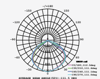
LUMINOUS INTENSITY DISTRIBUTION DIAGRAM
