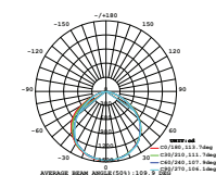
LUMINOUS INTENSITY DISTRIBUTION DIAGRAM
